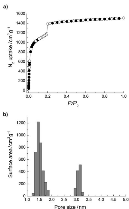
Figure 3. a) Nitrogen adsorption isotherm at 77 K for UCMC-1 (●, adsorption; ○, desorption). b) Pore size distribution calculated after fitting DFT models to argon gas adsorption data at 87 K.
